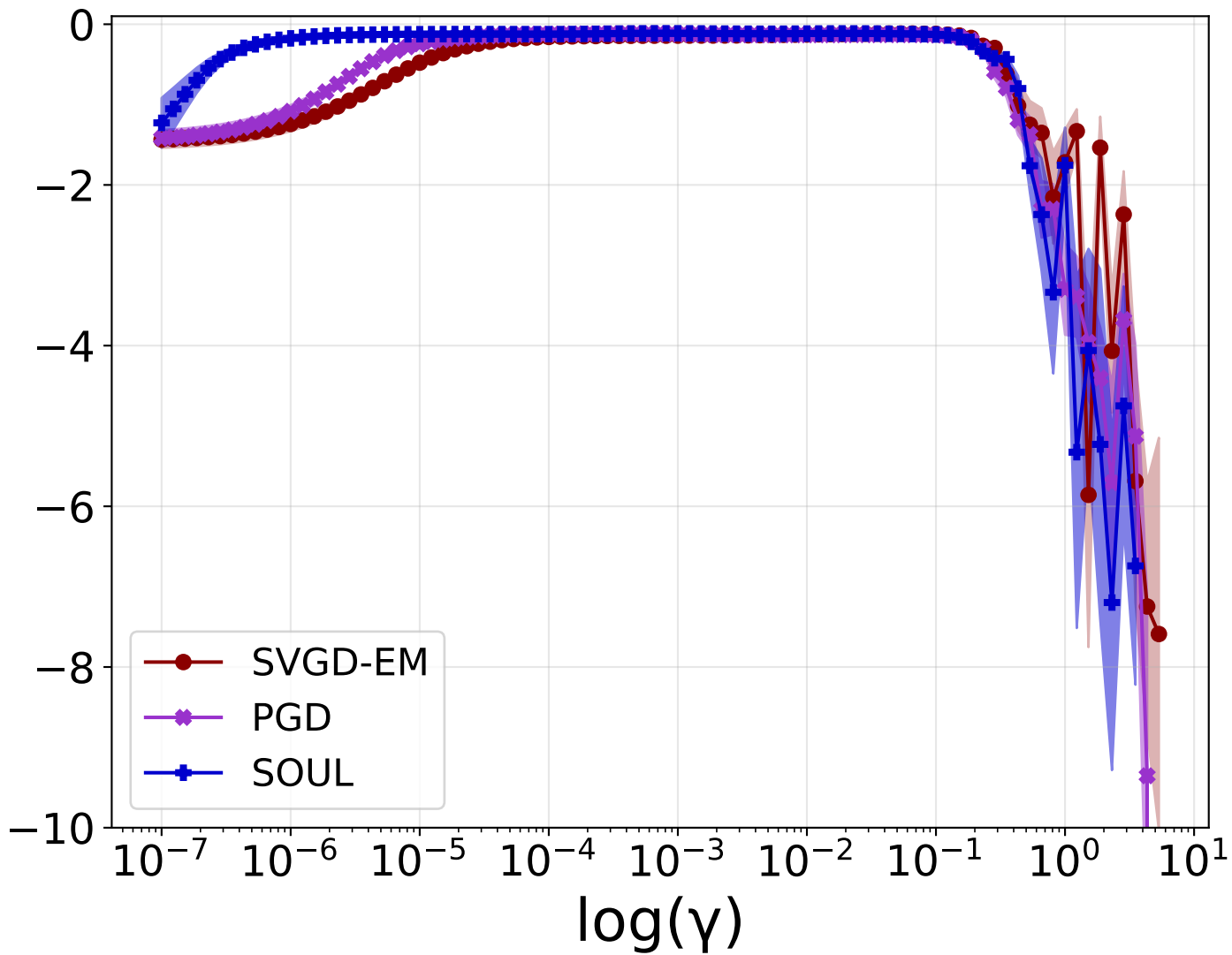
Log Predictive Density
